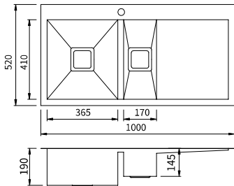
TOP4020D-SS Square Corner
