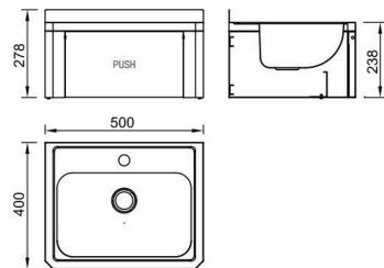
HWB-KO4 KNEE OPERATED BASIN
