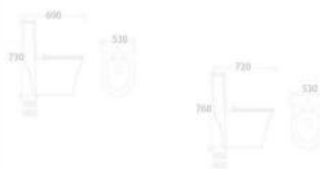
AMT2402 Siphonic One-piece Closet SIZE:720*530*760mm S-trap : 300/400mm Roughing in
