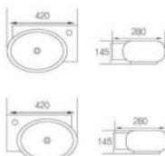
■ AMH1207L/1207R Wall-hung Basin Size: 420x280x145mm Wall-hung Installation
