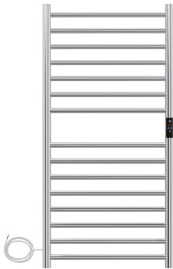
Model : SS105-15 Size (L X W X H) mm | 1000x 425 x 122 Size (L X W X H) in | 39.3 x 16.7 x 4.80 Power | 142.4 Watts
