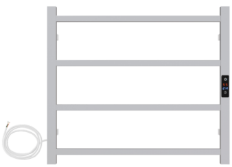
Model : SSS55TT-4 Size (L X W X H) mm | 520x 535 x 122 Size (L X W X H) in | 20.4 x 21.0 x 4.80 Power | 48.6 Watts
