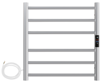
Model : SS66TT-6 Size (L X W X H) mm | 620x 600 x 122 Size (L X W X H) in | 24.4 x 23.6 x 4.80 Power | 70.2 Watts
