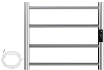
Model : SS56TT-4 Size (L X W X H) mm | 520x 600 x 122 Size (L X W X H) in | 20.4 x 23.6 x 4.80 Power | 48.6 Watts
