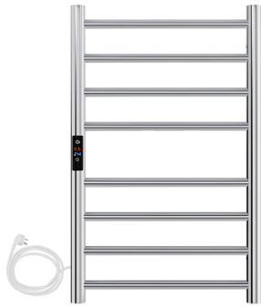
Model : SS85TT-8 Size (L X W X H) mm | 800x 500 x 122 Size (L X W X H)in | 31.4 x 19.6 x 4.80 Power | 61.2 Watts
