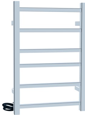
Model :SSS64-6 Size (L X W X H) mm | 600x 400 x 122 Size (L X W X H) in | 23.6 x 15.7 x 4.8 Power | 61.2 Watts
