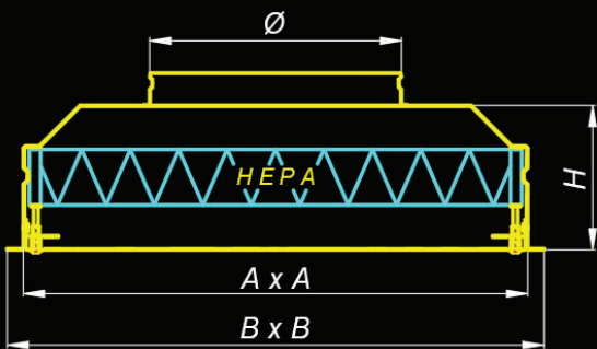
Diffuser A
