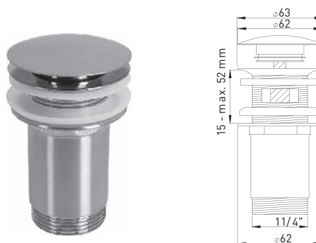
105748 Design drain waste 1 1/4" x Ø 63 mm Plug Ø 62 mm, lockable brass stainless steel look with overview slot
