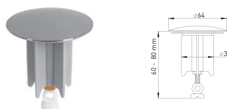
100417 Universal brass big plug 1½" Plate Ø 64 mm, suitable for all brands White seal, stainless steel look
