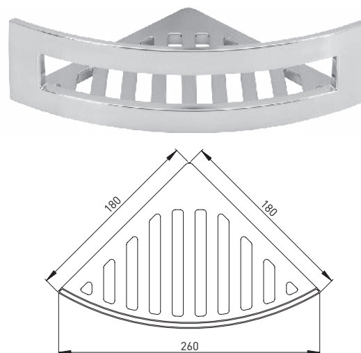
104664 Corner sponge basket closed complete with fastening stainless steel look 260 mm x 180 mm
