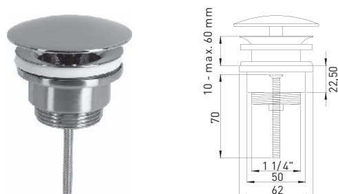
106442 Design universal waste 1 1/4" x Ø 63 mm plug Ø 72 mm, round, stainless steel look, not lockable
