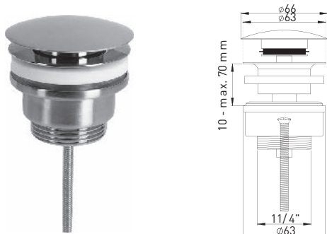
106723 Design universal waste 1 1/4" x Ø 63 mm plug Ø 66 mm, round, stainless steel look, lockable
