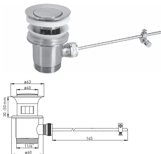
100447 Brass 1½" pop-up waste with standard eccentric plug brass stainless steel look
