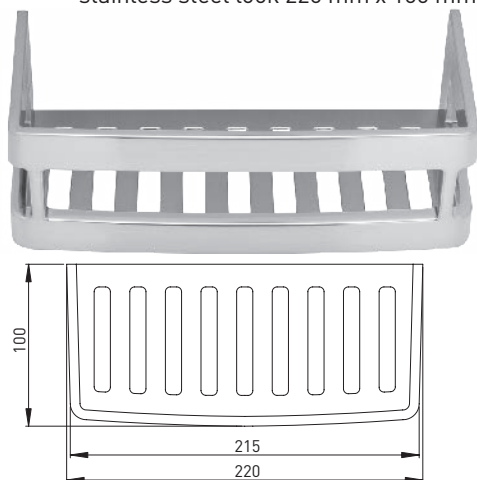
104612 Sponge basket closed complete with fastening stainless steel look 220 mm x 100 mm
