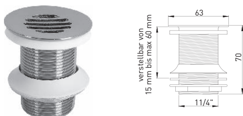
107691 Shaft waste 1 1/4" x Ø 63 mm with screen inlet, without overflow slot Shaft length: 70 mm brass stainless steel look
