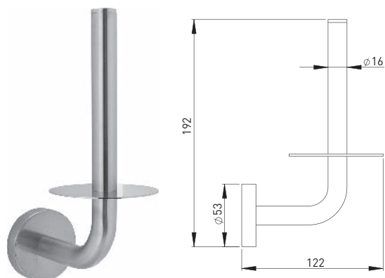
210826 Reserve toilet paper holder for one roll brass stainless steel look
