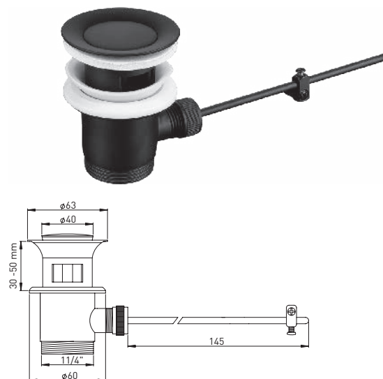
102605 Brass 1 1/4" pop-up waste with standard eccentric plug brass mat black
