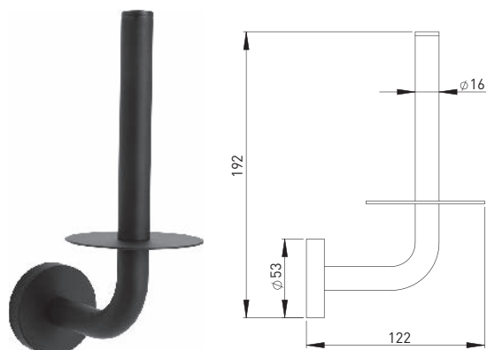
210800 Reserve toilet paper holder for one roll brass mat black
