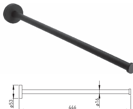
211518 1-armed towel holder brass mat black
