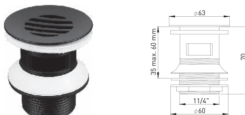
108462 Shaft waste 1 1/4" x Ø 63 mm with screen inlet, with overflow slot Shaft length: 70 mm brass mat black
