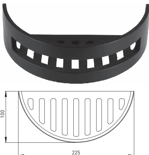
104599 Sponge basket closed complete with fastening mat-black 225 mm x 100 mm
