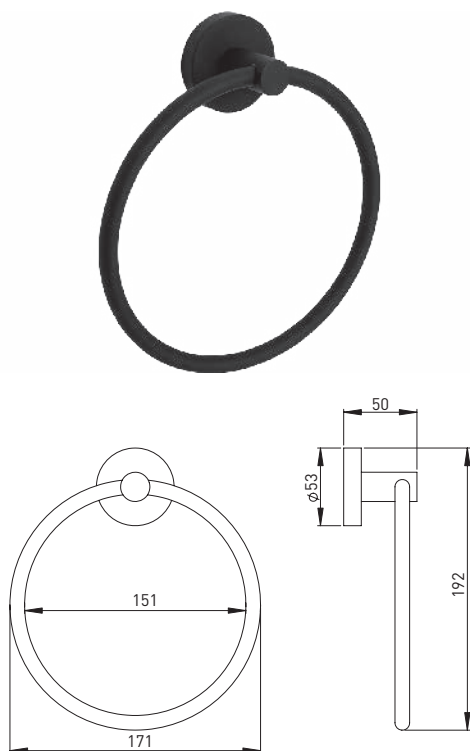
211561 Towel ring brass mat black
