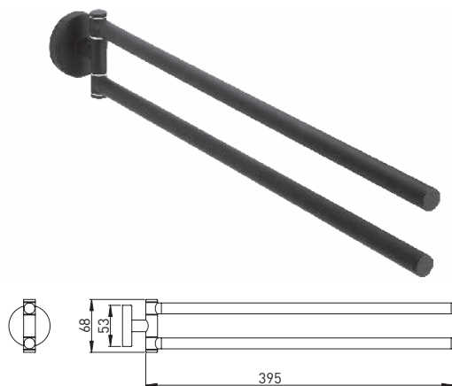
211445 2-armed towel holder brass mat black
