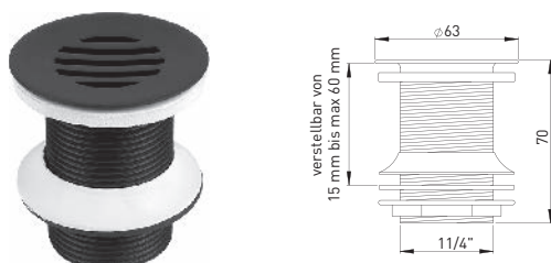
107663 Shaft waste 1 1/4" x Ø 63 mm with screen inlet, without overflow slot Shaft length: 70 mm brass mat black
