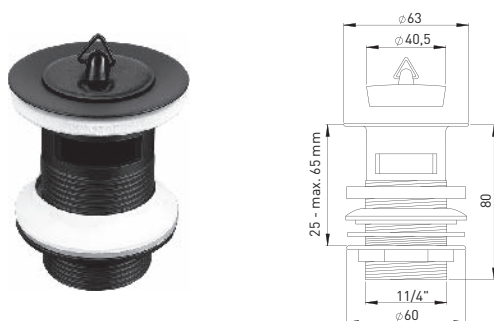
108392 Shaft waste 1 1/4" x Ø 63 mm with overflow, complete with plug Shaft length 80 mm, brass, mat black
