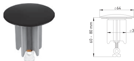
102533 Universal brass big plug 1 1/4" Plate Ø 64 mm, suitable for all brands White seal, brass mat black
