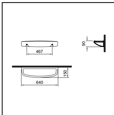
WISA ABLAGE 64 CM
