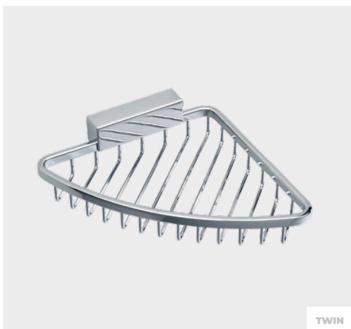
IRIS² Schwammkorb Eck I411-0000 B=164 mm, T=176 mm, H=44 mm
