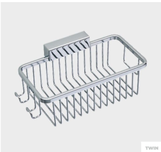
IRIS 2 Shampookorb Wand I450-0000 B=213mm, T=116 mm, H=80 mm
