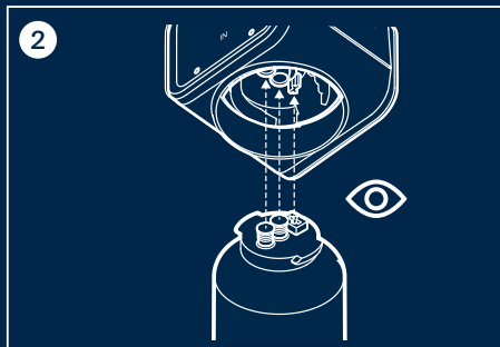
2. Remove the lid from new filter and assemble it to the head (rotating 90 degrees).
