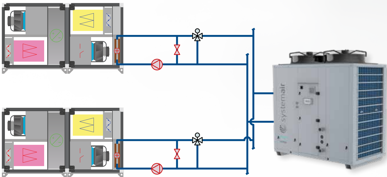
Example installation of one AHU master, one AHU slave and one SYSAQUA R32 chiller/heat pump
