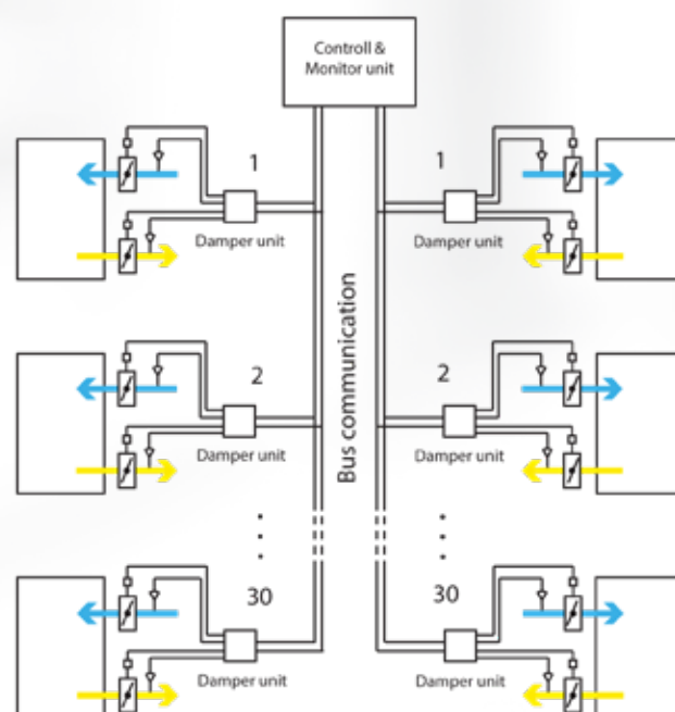
Example of a complete fire damper controls system
