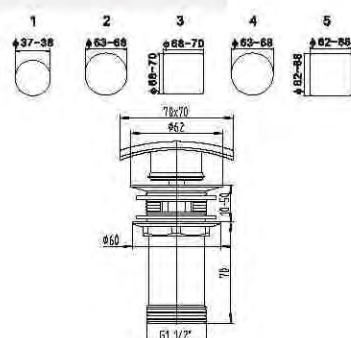
Basin click-clack pop-up
