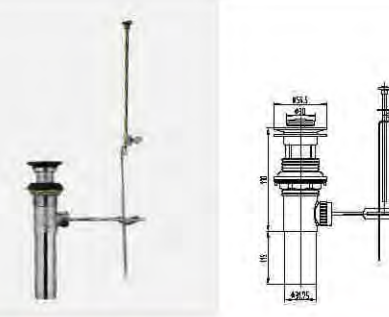
Basin click-click pop-up
