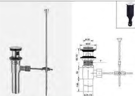
Basin click-click pop-up
