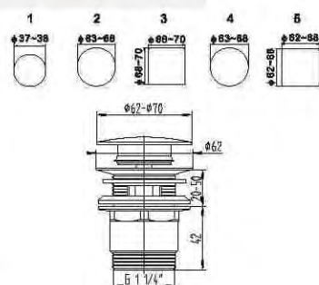
Basin click-clack pop-up
