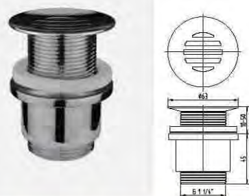
Free flow drain waste
