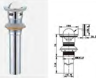
Basin flip waste
