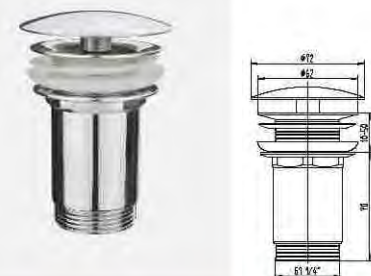
Free flow drain waste
