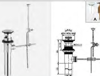
Basin click-click pop-up
