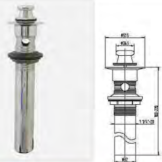
Basin click click pop-up
