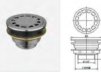
Free flow drain waste
