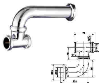
Item no Material Size/mm G30165 00 Brass 1 1/2 G30160 00 Brass 1 1/4
