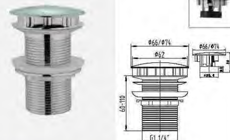
Free flow drain waste
