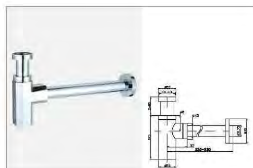
Bottle siphon with rosette
