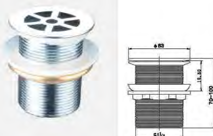
Free flow drain waste
