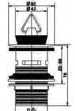
Brass waste for wash basin 1 1/4", with overflow brass plug
