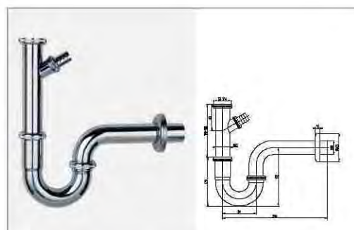
P-siphon with rosette
