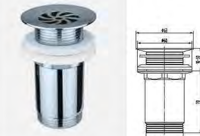
Free flow drain waste
