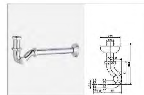
P-siphon with rosette
