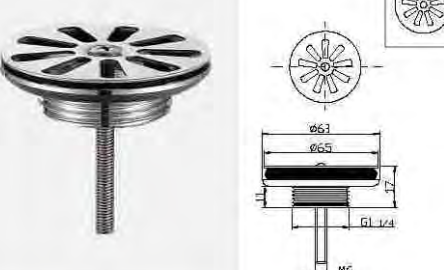
Free flow drain waste
