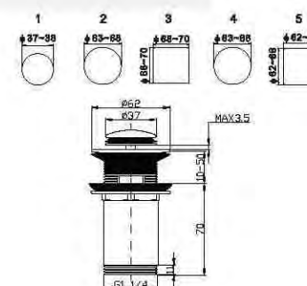
Basin click-clack pop-up
