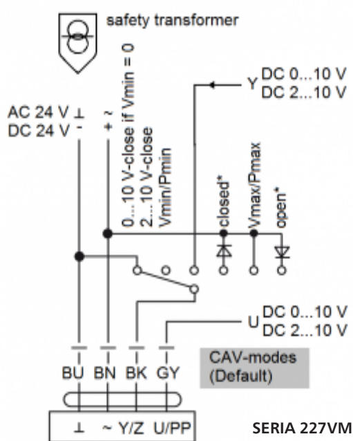
Connection diagram RAVAV-G
