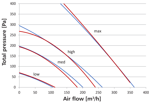
HRU-MinistAIR-325 — SUPPLY — EXHAUST
