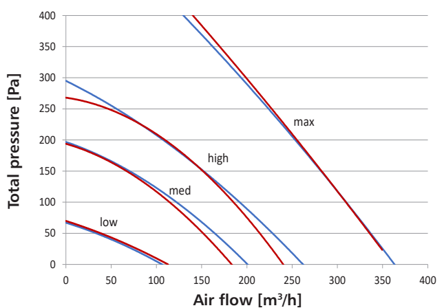
HRU-MinistAIR-LS-325E — SUPPLY — EXHAUST
