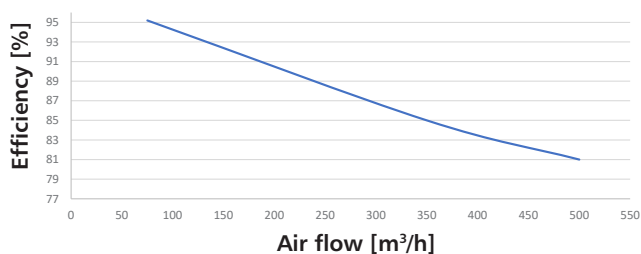
Performance curve HRU-SlimAIR-500
