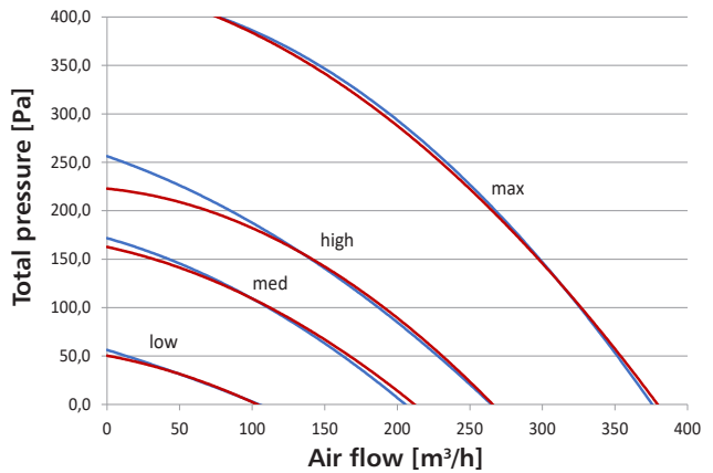
HRU-MinistAIR-L-325-E — SUPPLY — EXHAUST
