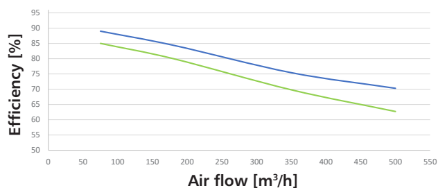
Performance curve Heat (—) and moisture recovery (—) HRU-SlimAIR-500E
