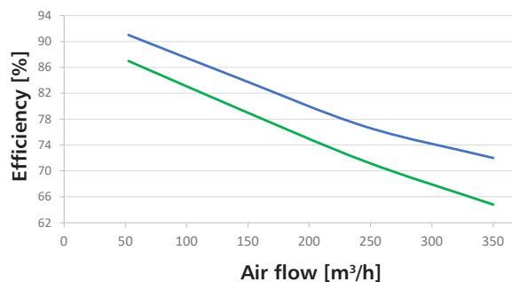
Performance curve Heat (—) and moisture recovery (—) HRU-SlimAIR-350E
