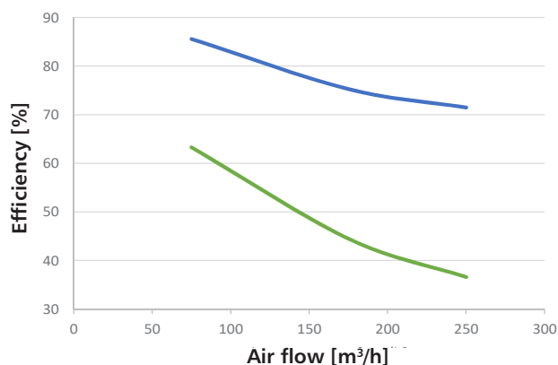
Performance curve Heat (—) and moisture recovery (—) HRU-SlimAIR-250E-H
