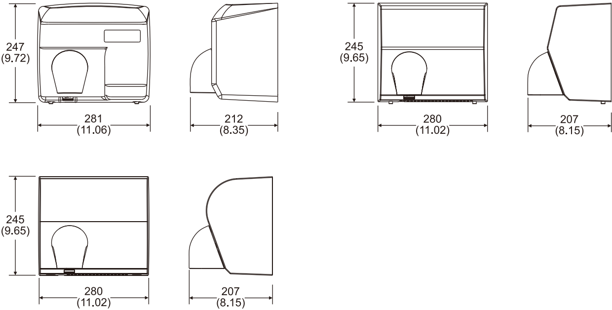
DIM'S mm(inch)
