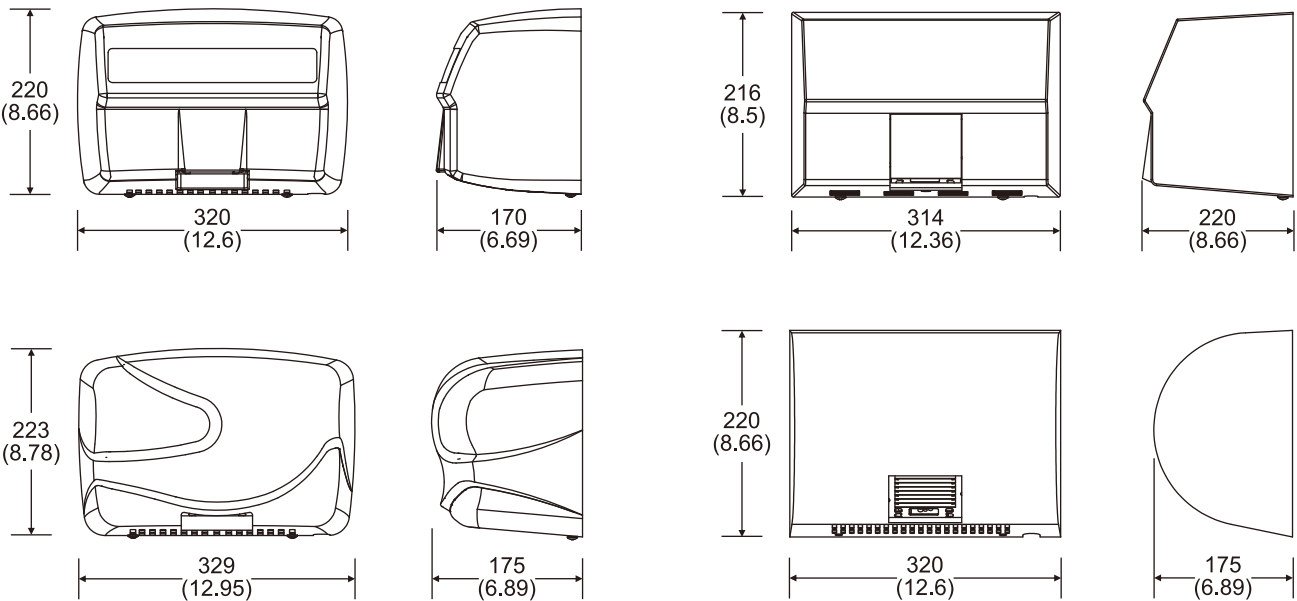
DIM'S mm(inch)
