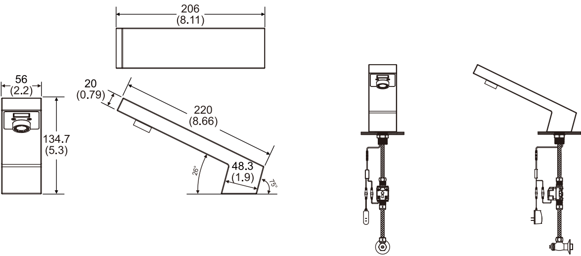
Mounted on a Single-Hole Lavatory or Deck (Ø35)
