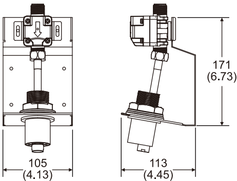
Fixing plate may be required for installation behind the mirror
