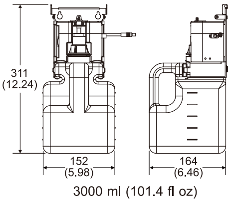
DIM'S mm(inch)
