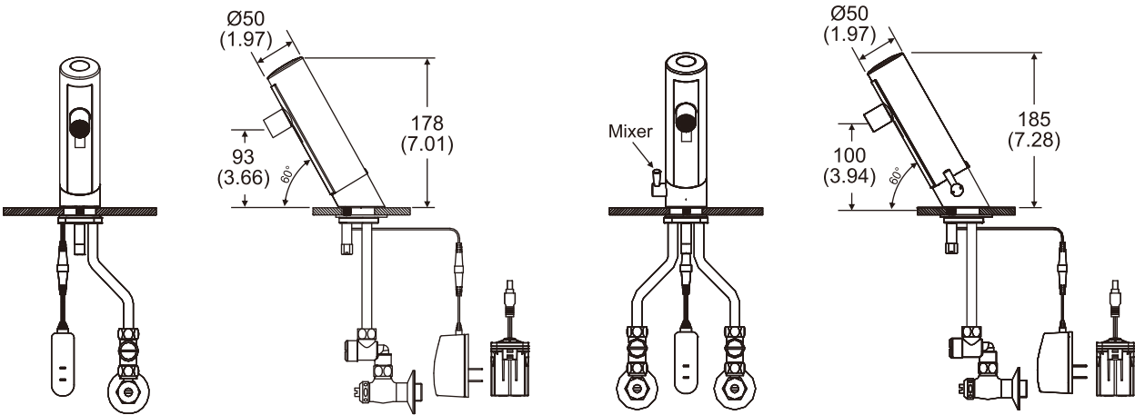
Mounted on a Single-Hole Lavatory or Deck (Ø28 - Ø45)
