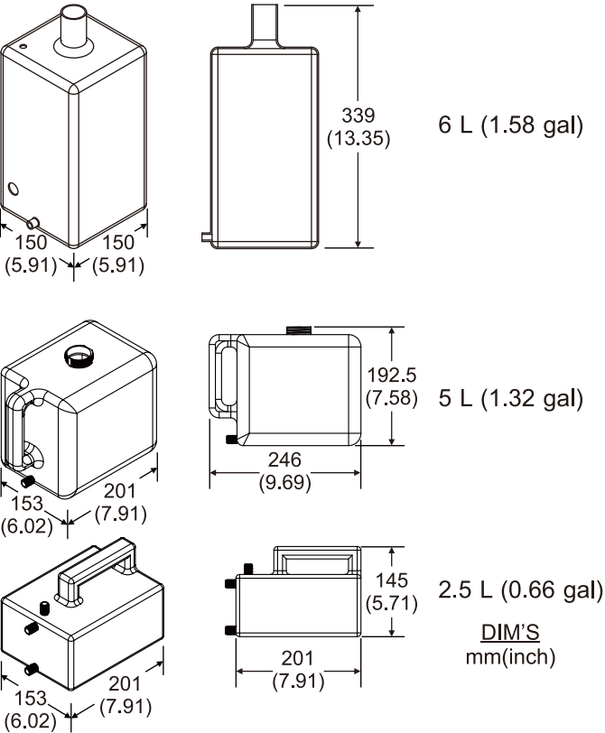
Soap Tank
