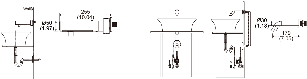
Mounted on a UT Wall (Ø35)
