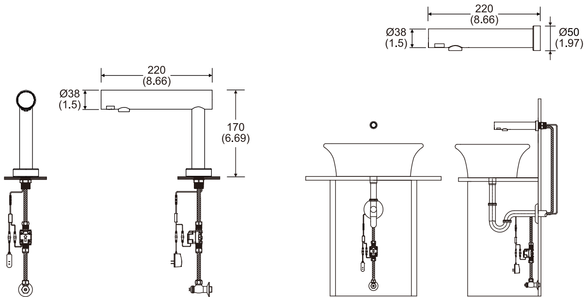
DIM'S mm(inch)
