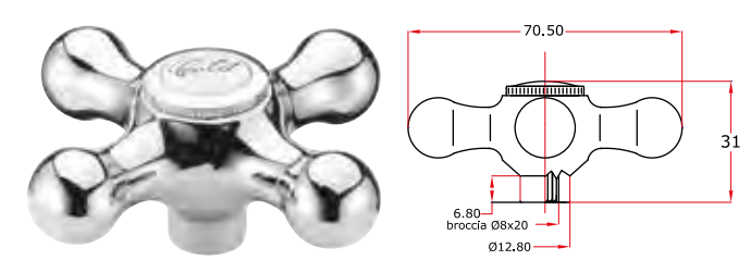
Art. 114 Maniglia Harmony
