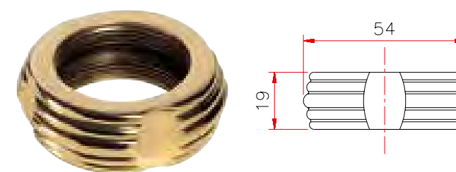
Art. 055 Anello Australia
