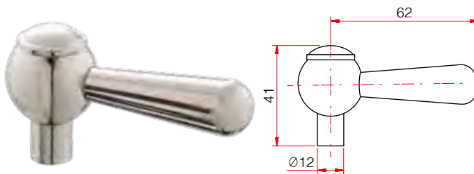
Art. 215 Leva Pipa C
