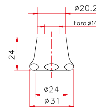
Art. 305 Coprivitone Export
