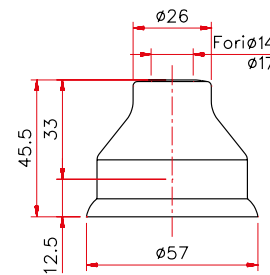
Art. 369 Cappuccio Silver
