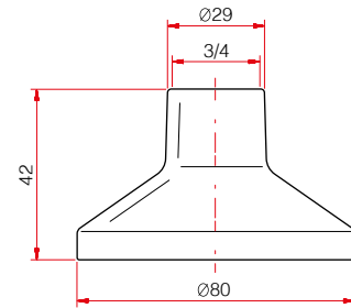
Art. 364 Cappuccio Napoli Ø 80
