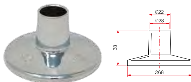
Art. 347 Cappuccio Incas
