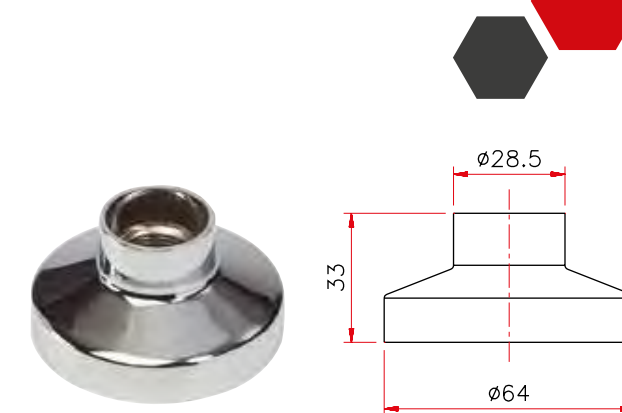
Art. 359 Cappuccio Antony
