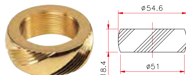
Art. 023 Anello Austria
