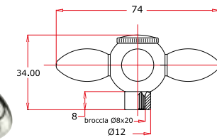
Art. 131 Maniglia Alessia
