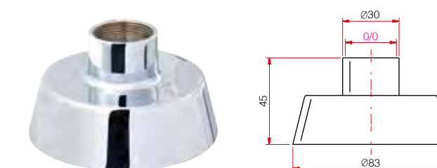
Art. 362 Cappuccio Milano Ø 84
