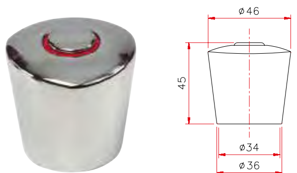
Art. 177 Maniglia Martin
