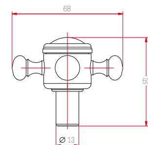
Art. 128 Maniglia Victoria
