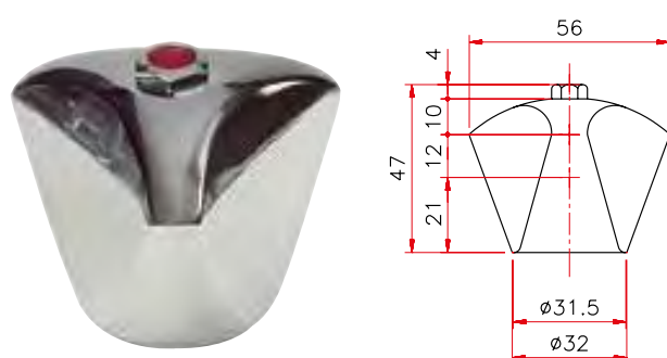
Art. 175 Maniglia Globo
