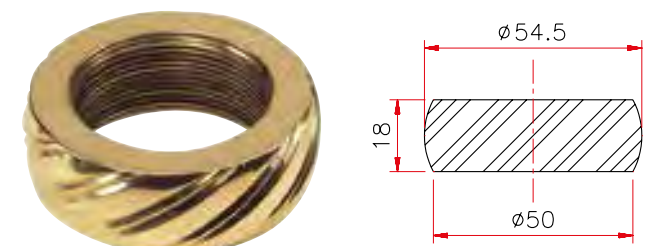
Art. 041 Anello Africa
