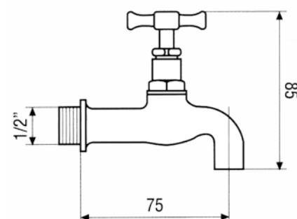
Art. 900 Rubinetto 1/2" portagomma Robinet 1/2" porta-tuyau Tap 1/2" with rubber pipe holder
