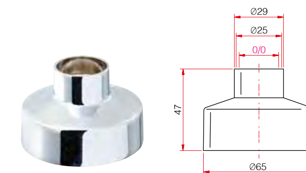
Art. 360 Cappuccio Mark Ø 66
