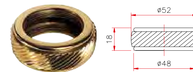
Art. 057 Anello India
