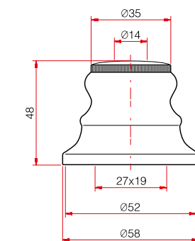
Art. 385 Cappuccio Charlotte
