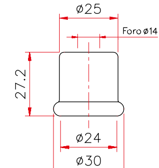
Art. 311 Coprivitone Tondo B
