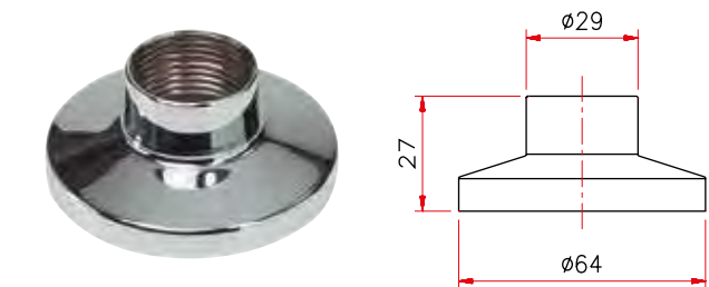
Art. 357 Cappuccio Frank
