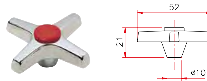
Art. 101 Maniglia Vanity
