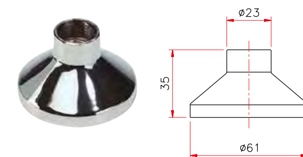
Art. 363 Cappuccio Lima
