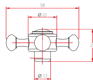
Art. 124 Maniglia Edward
