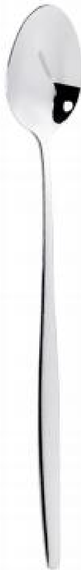
Ice spoon Length: 198mm Weight: 28.8g Thickness: 3mm
