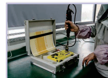
Screwdriver Torque Checking Tester
