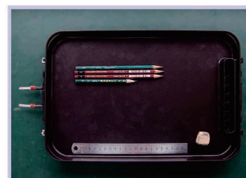
Pencil Hardness Test
