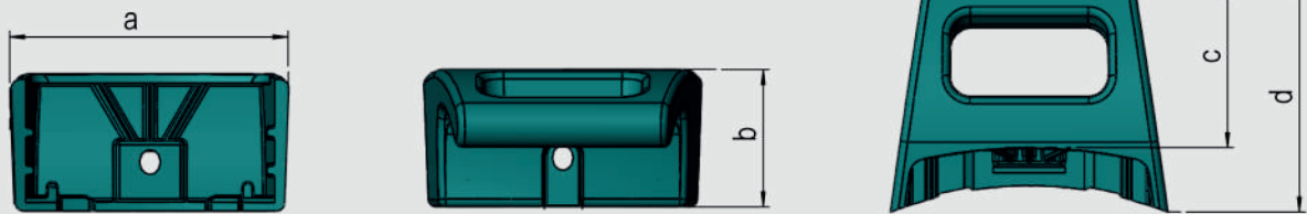
asa lateral / side handle
