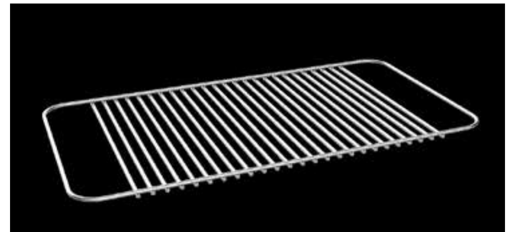
FUEGO extra BBQ grid in stainless steel Item nr: 7340315-1 Size: 27 x 50 cm, 8 mm frame, 5 mm grid
